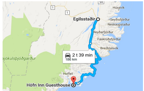
The leg day 5, on July 15, looked like this. The road goes over the mountain. It was a dirt road and there was thick fog and heavy rain, so it was slow going over the mountains. It suited us that we had a good time that day.
